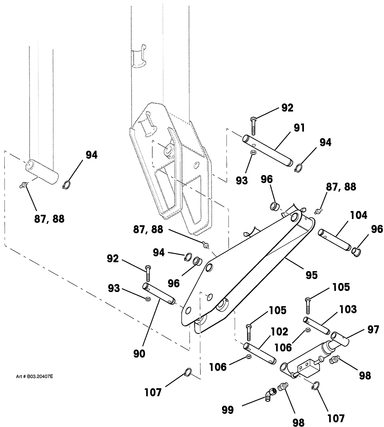
Lower Leveling Arm
